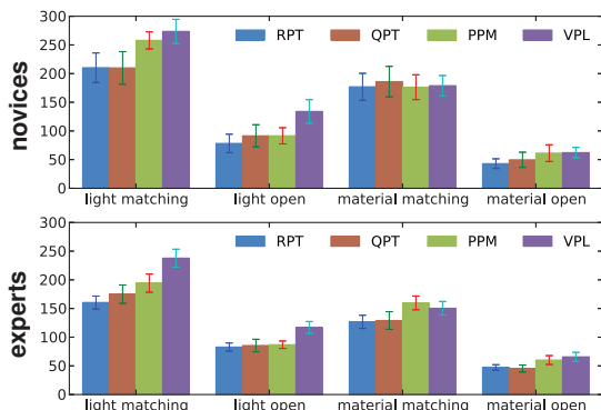
Figure 4: Average time to completion. Subjects generally finished sooner using one of the path tracers than using the VPL algorithm.
