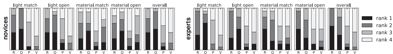
Figure 9: Algorithm rankings ( R = RPT , Q = QPT , P = PPM , V = VPL ). Two path tracers were ranked higher than the other two methods in the overall ranking and in the two lighting trials.
