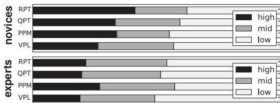
Figure 7: Proportion of time users spent at each resolution. Experts spend less time at high resolution.
