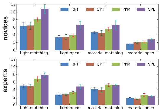
Figure 6: Average time between user interactions in seconds. For matching tasks, it is the average interval between two clicks on the slider. For open tasks, it is the average interval between changing the designs. Experts take slightly less time than novices.
