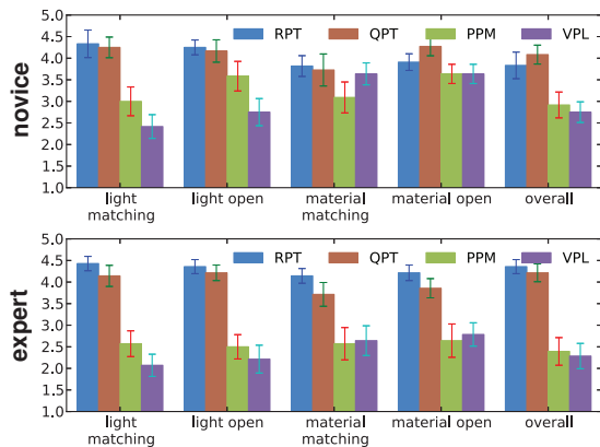
Figure 8: Algorithm ratings. Experts have a stronger preference toward path tracing algorithms.
